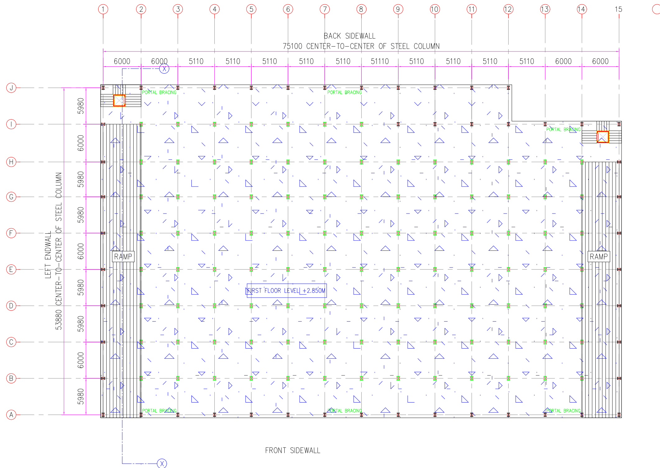
FLOOR PLAN @ LVL.+2.85m, 5.7m, 8.55m, 11.4m, 14.25m, 17.1m, 19.95m, 22.8m
